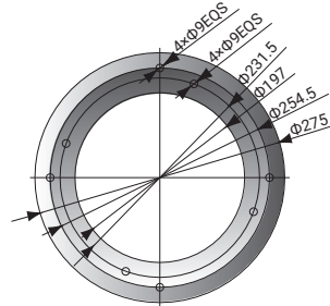
SHR-6U-S~SHR-24U-ST Basisflansch
