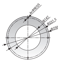
SHR-3U Basisflansch
