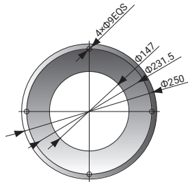
SHR-3U-ST Basisflansch
