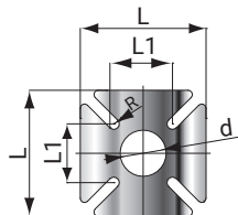
SHR-U-EST Basisflansch
