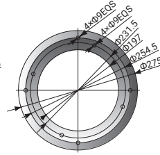
SHR-6U-S~SHR-24U-S Basisflansch
