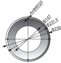
SHR-3U-S Basisflansch
