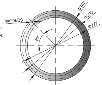
SHR-36U-ST~SHR-48U-ST Basisflansch
