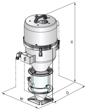
SHR-U-ES
