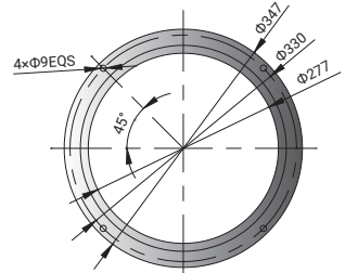
SHR-36U-S~SHR-96U-S Basisflansch
